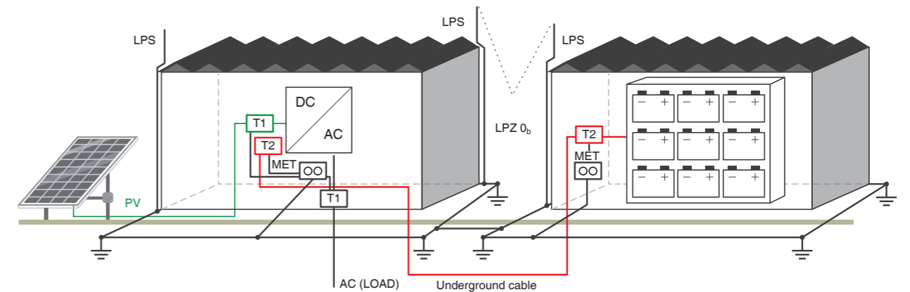
Scenario 2: BESS with separate concrete structures for AC/DC converter and the battery located nearby. The separation distance between the LPS and the BESS equipment is maintained. Common grounding, DC cable routed underground in a protected area (LPZ 0b). T2 DC SPDs required; T1/T2 recommended. If the DC cable length is <10m, only one DC SPD (either at the inverter or the battery) is required. The same approach counts for metal constructions.
