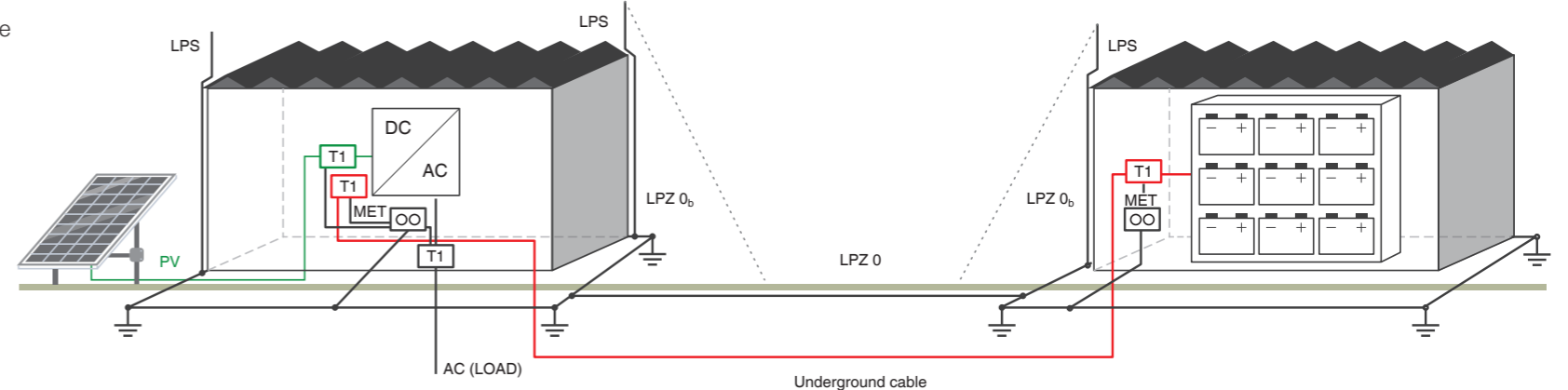
Scenario 3: BESS with separate concrete structures for AC/DC converter and battery. The separation distance between the LPS and the BESS equipment is maintained. Common or separated grounding, DC cable is routed above ground or underground in a cable trench in the LPZ 0 area. T1 DC SPDs are required; T1/2 is recommended. The same approach counts for metal constructions.
