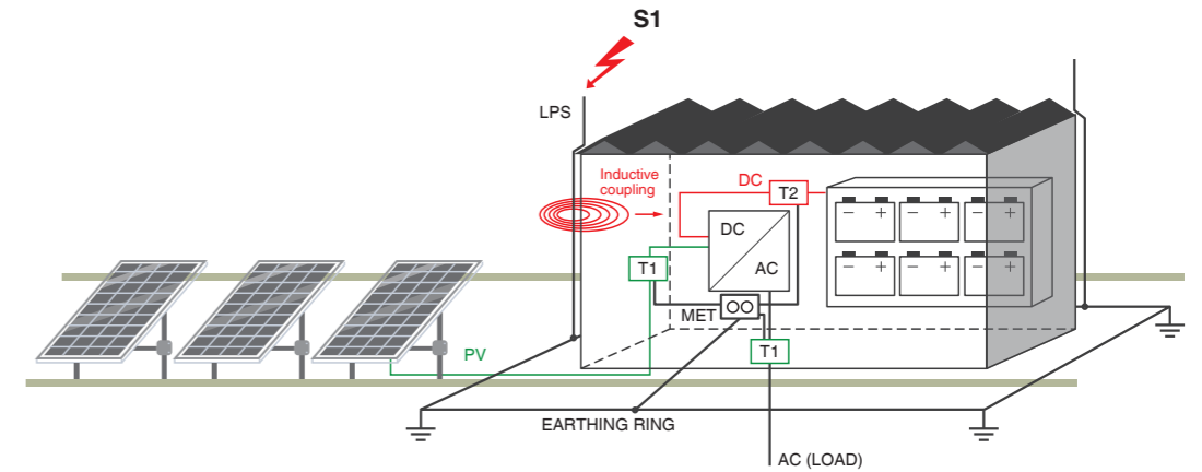
Scenario 1: BESS with common concrete structure for AC/DC converter and battery. Separation distance between the LPS and the BESS equipment is maintained. One T2 DC SPD needs to be installed to protect against the influence of the S1 event (inductive coupling). In the case of metal construction with lightning current sharing via the housing (walls), the inductive coupling is reduced, and the DC SPD may be eliminated.
